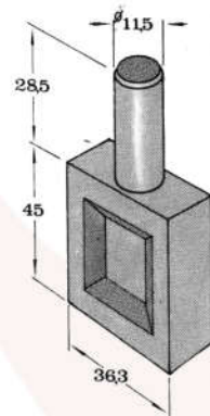
NYL 201 Guia Superior Nylon Preto
