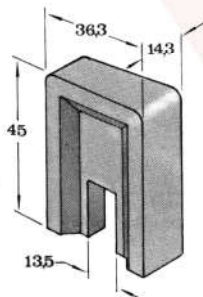
NYL 202 Guia Inferior Nylon Preto
